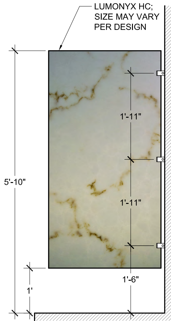
URINAL SCREEN ELEVATION SCALE: 3/4" = 1'
