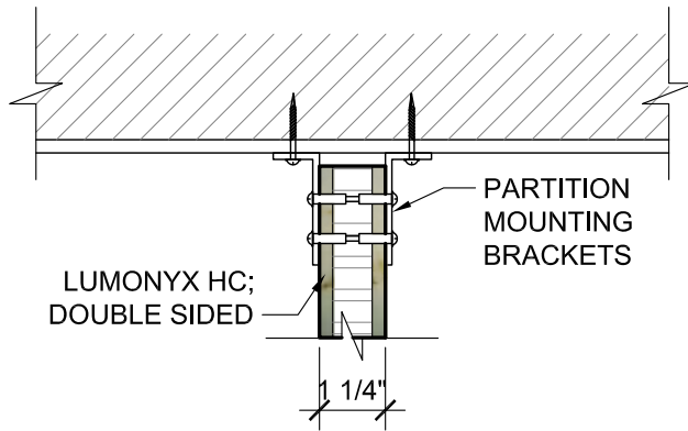
SCREEN MOUNTING DETAIL SCALE: 3" = 1'
