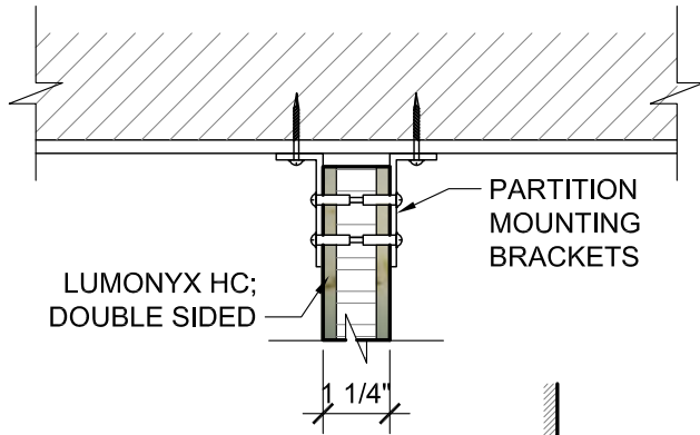
TOILET PARTITION WALL DETAIL SCALE: 3" = 1'
