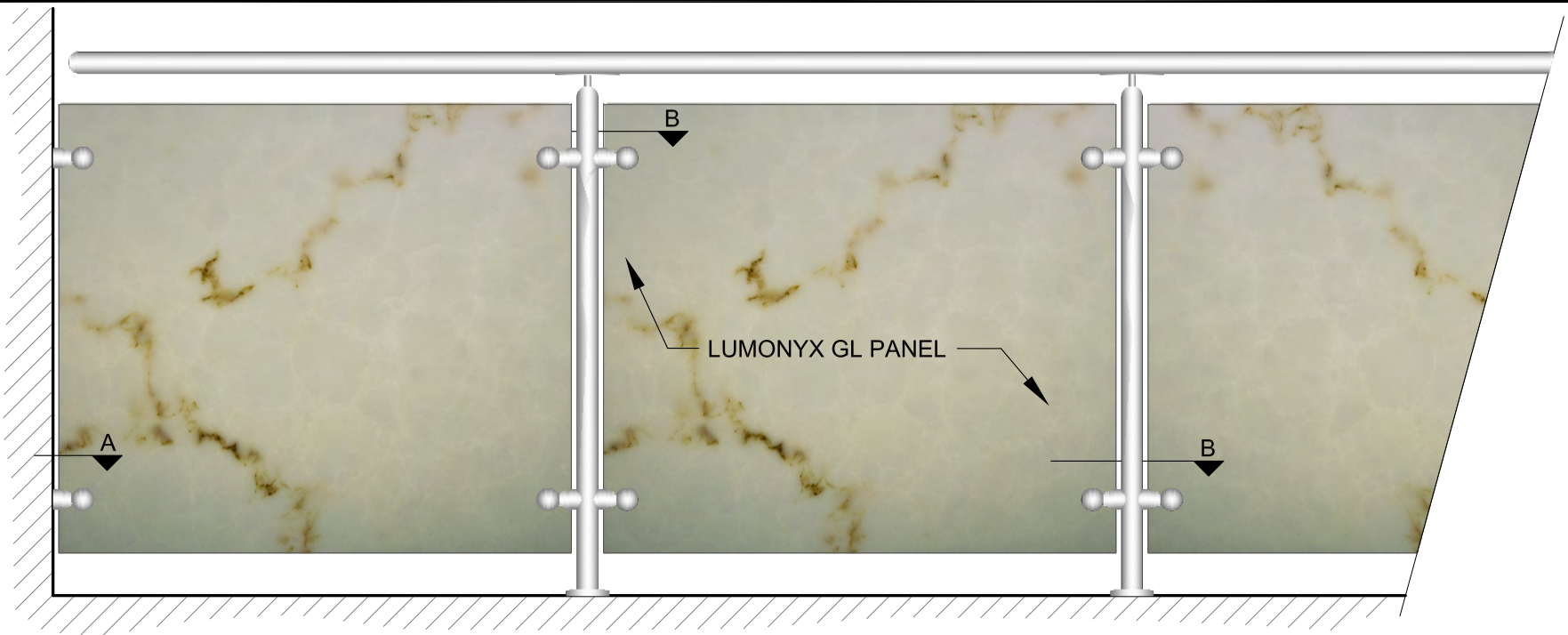
RAILING ELEVATION SCALE: 3/16" = 1'
